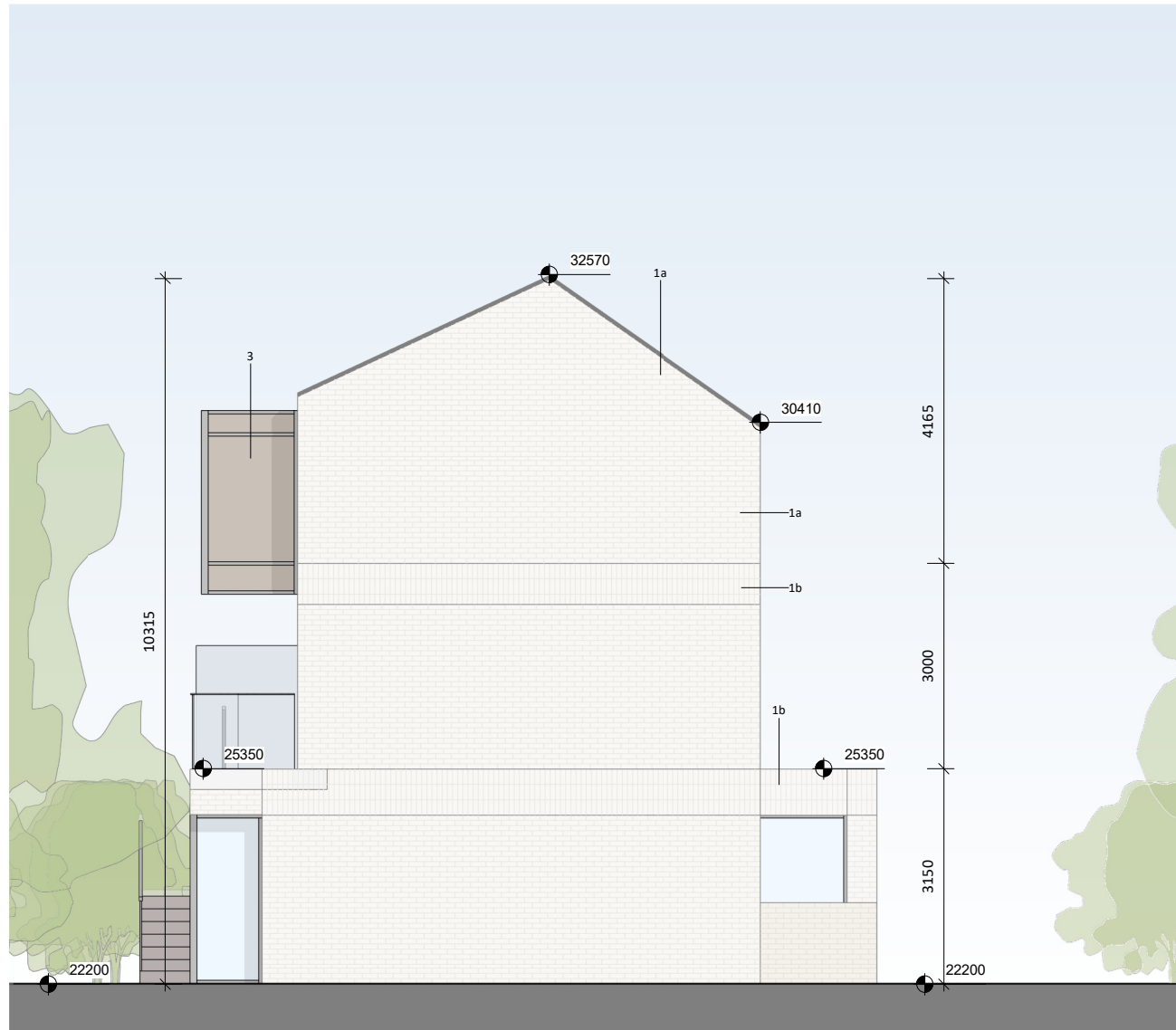
2 T05 North Elevation 1 : 100
