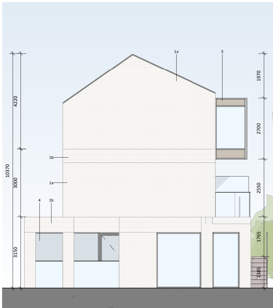
4 T05 South Elevation 1 : 100
